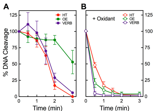
Figure 8. Olive metabolites inhibit topoisomerase II \alpha when incubated with the enzyme prior to DNA. The effects of hydroxytyrosol (HT; red), oleuropein (OE; green), and verbascoside (VERB; purple) are shown. Metabolites were incubated with the human enzyme in the absence of oxidant (1 mM metabolite, filled circles, left) or in the presence of 10 \mu M K 3 Fe(CN) 6 (10 \mu M metabolite, empty circles, right). DNA cleavage levels were calculated relative to a control reaction mixture to which the metabolite was added after the addition of DNA to assay mixtures. Error bars represent standard deviations of at least three independent experiments.
