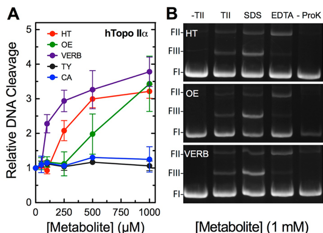
Figure 3. Olive metabolites enhance DNA cleavage mediated by human topoisomerase II \alpha . (A) The effects of hydroxytyrosol (HT; red), oleuropein (OE; green), verbascoside (VERB; purple), caffeic acid (CA; blue), and tyrosol (TY; black) on DNA cleavage mediated by topoisomerase II \alpha are shown. DNA cleavage levels were calculated relative to a control reaction mixture that contained no metabolite. Error bars represent standard deviations for three independent experiments. (B) DNA cleavage induced by hydroxytyrosol (top), oleuropein (middle), or verbascoside (bottom) is reversible and protein-linked. Ethidium bromide-stained agarose gels are shown. Assay mixtures contained DNA with olive metabolites in the absence of enzyme (–TII), topoisomerase II \alpha with DNA in the absence of olive metabolites (TII), or complete reactions stopped with SDS prior to the addition of EDTA (SDS). To determine whether the reaction was reversible, EDTA was added prior to SDS (EDTA). To determine whether the cleaved DNA was protein-linked, proteinase K treatment was omitted (–ProK). The mobilities of negatively supercoiled DNA (form I; FI), the nicked circular plasmid (form II; FII), and linear molecules (form III; FIII) are indicated. Gels are representative of three independent experiments.
