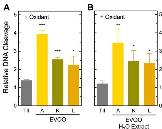
Figure 12. Extra virgin olive oils enhance DNA cleavage mediated by topoisomerase II \alpha . The effects of extra virgin olive oils (EVOOs) or an EVOO H 2 O extract on DNA cleavage mediated by the human type II enzyme are shown in panels A and B, respectively. Olive oils [Ultra Arbonsana (A, yellow), Ultra Koroneiki (K, green), or Lucini Select (L, brown)] or extracts from these oils were included in reaction mixtures at final concentrations of 10% (v/v) in the presence of 10 \mu M K 3 Fe(CN) 6 . Results for reaction mixtures that contained no oils or extracts but contained oxidant (TII; gray) are shown. DNA cleavage levels were calculated relative to a control reaction mixture that contained no olive oil or oxidant. Error bars represent the standard deviation of at least three independent experiments. Statistically significant differences are noted with asterisks (* p < 0.05; ** p < 0.001; *** p \leq 0.0001).
